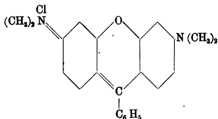
Rosamin (Chlorid).
